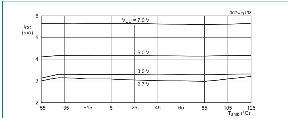
Fig 3. Supply current versus ambient temperature
