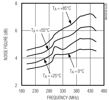
VHF-H NOISE FIGURE vs. FREQUENCY
