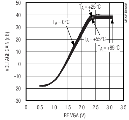
VHF-H VOLTAGE GAIN vs. RF VGA VOLTAGE
