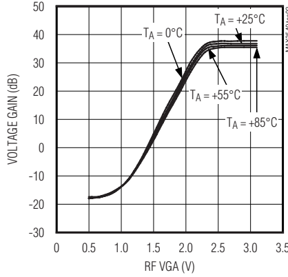
VHF-L VOLTAGE GAIN vs. RF VGA VOLTAGE
