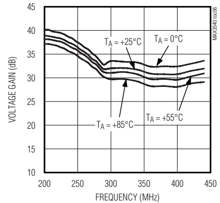
VHF-H VOLTAGE GAIN vs. FREQUENCY
