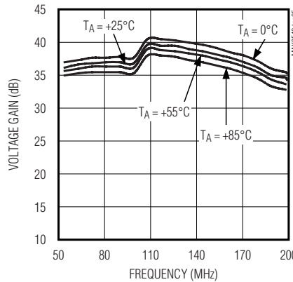
VHF-L VOLTAGE GAIN vs. FREQUENCY
