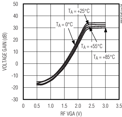
UHF VOLTAGE GAIN vs. RF VGA VOLTAGE
