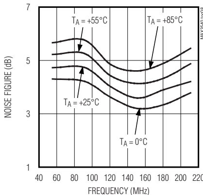
VHF-L NOISE FIGURE vs. FREQUENCY
