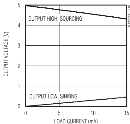
RECEIVER OUTPUT (RO1) VOLTAGE vs. LOAD CURRENT
