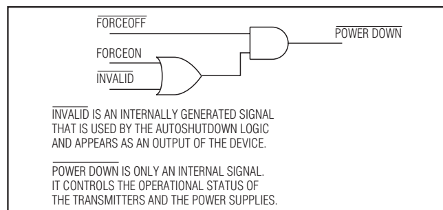
Figure 3c. MAX3221E/MAX3223E/MAX3243E AutoShutdown Logic
