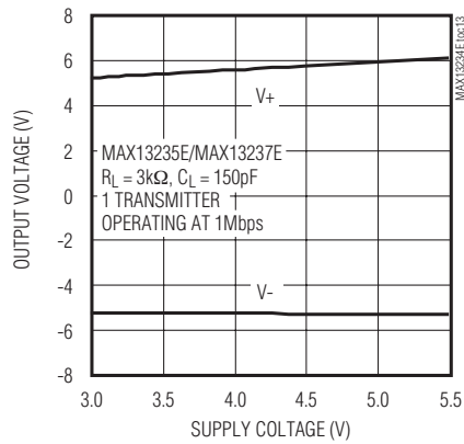
TRANSMITTER OUTPUT VOLTAGE vs. SUPPLY VOLTAGE
