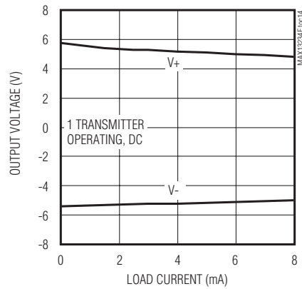
TRANSMITTER OUTPUT VOLTAGE vs. LOAD CURRENT
