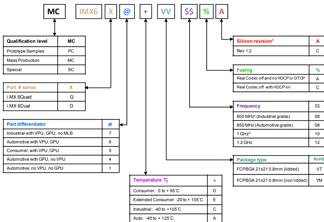
Figure 1. Part Number Nomenclature—i.MX 6Quad and i.MX 6Dual
