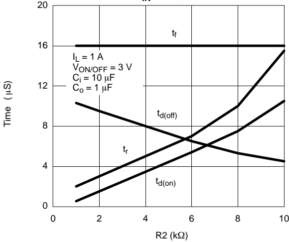
Switching Variation R2 @ V_IN = 10 V, R1 = 300 kΩ
