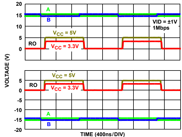
FIGURE 20. ±15V RECEIVER PERFORMANCE (ISL32433E, ISL32435E)
