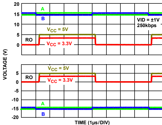
FIGURE 19. ±15V RECEIVER PERFORMANCE (ISL32430E, ISL32432E, ISL32437E)
