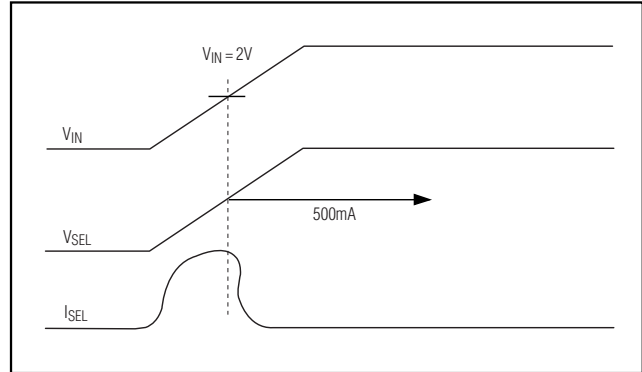
Figure 3. MAX4772 Power-Up Sequence ( V_{SEL} and V_{IN} Rise Simultaneously)
