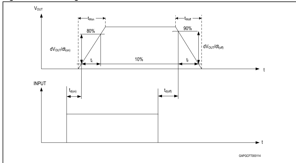
Figure 8. Switching characteristics
