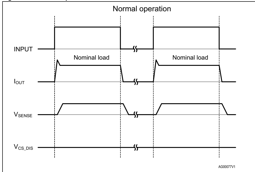
Figure 11. Normal operation
