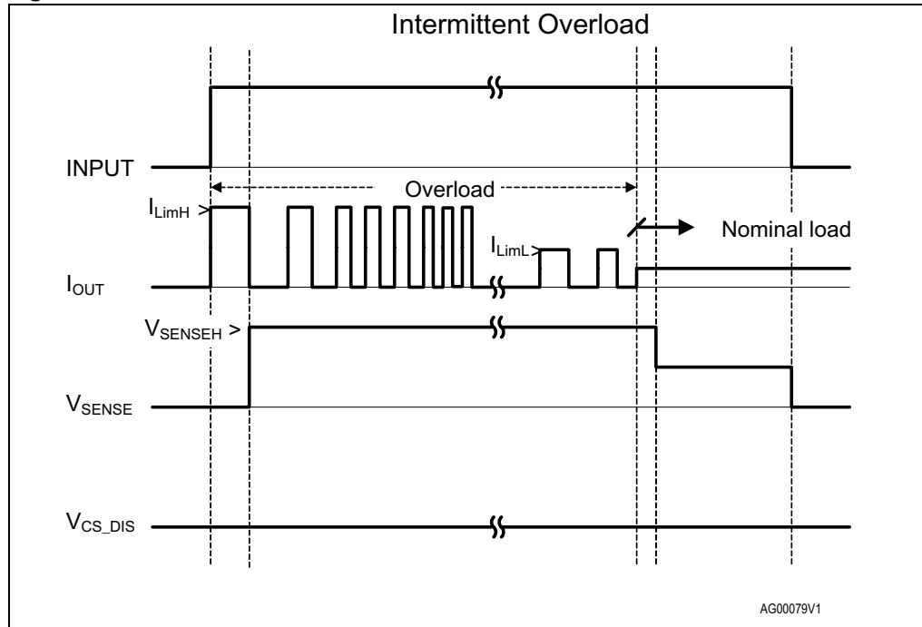
Figure 13. Intermittent overload
