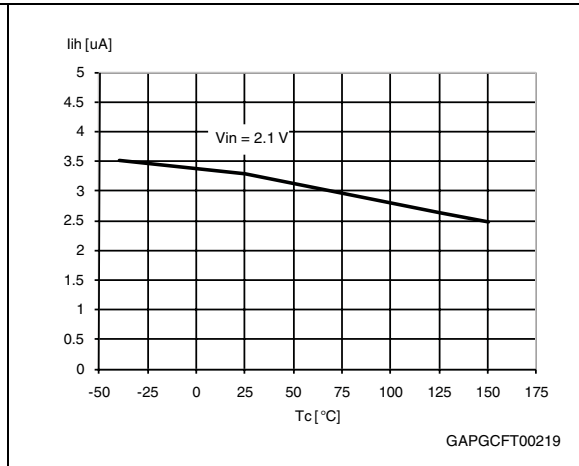
Figure 20. Input high level
