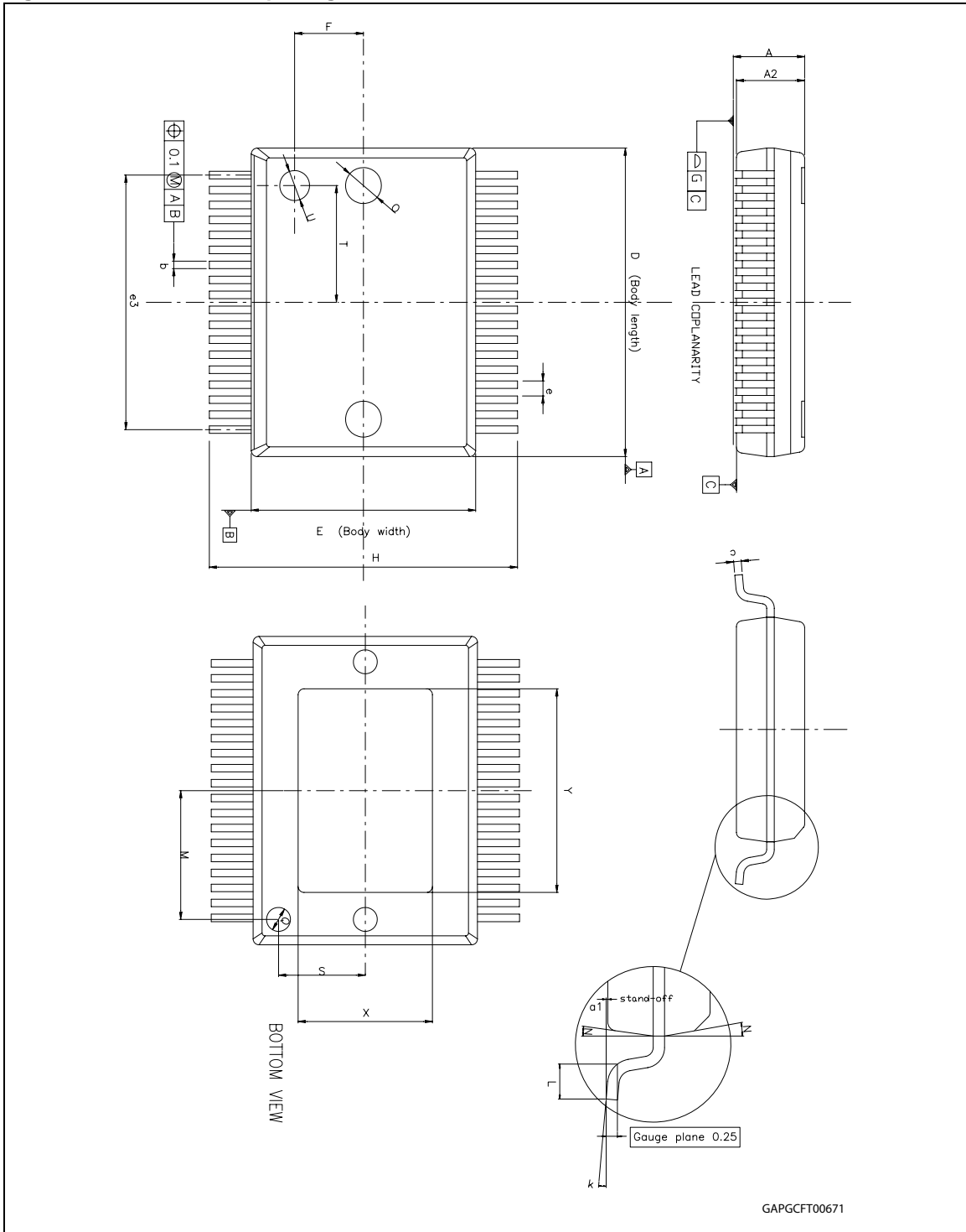
Figure 39. PowerSSO-36 package dimensions
