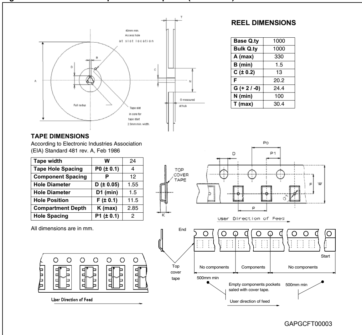
Figure 41. PowerSSO-36 tape and reel shipment (suffix "TR")
