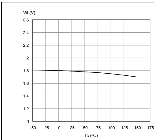
Figure 10. Input low level voltage
