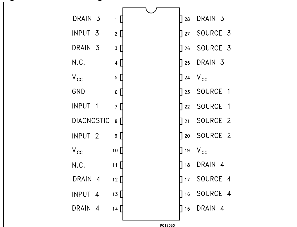
Figure 2. Connection diagram
