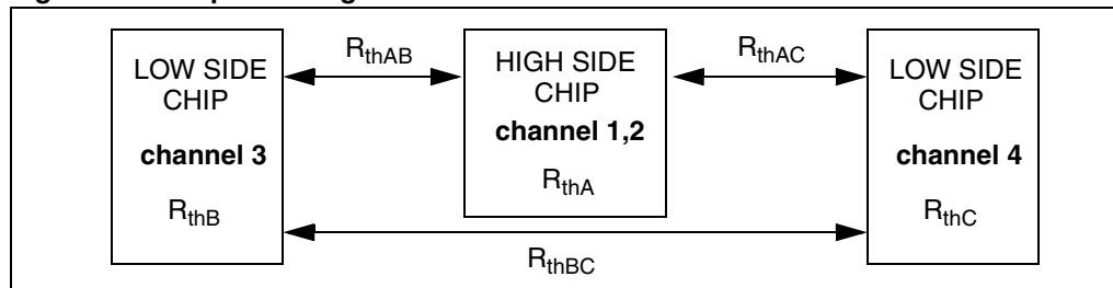
Figure 48. Chipset configuration
