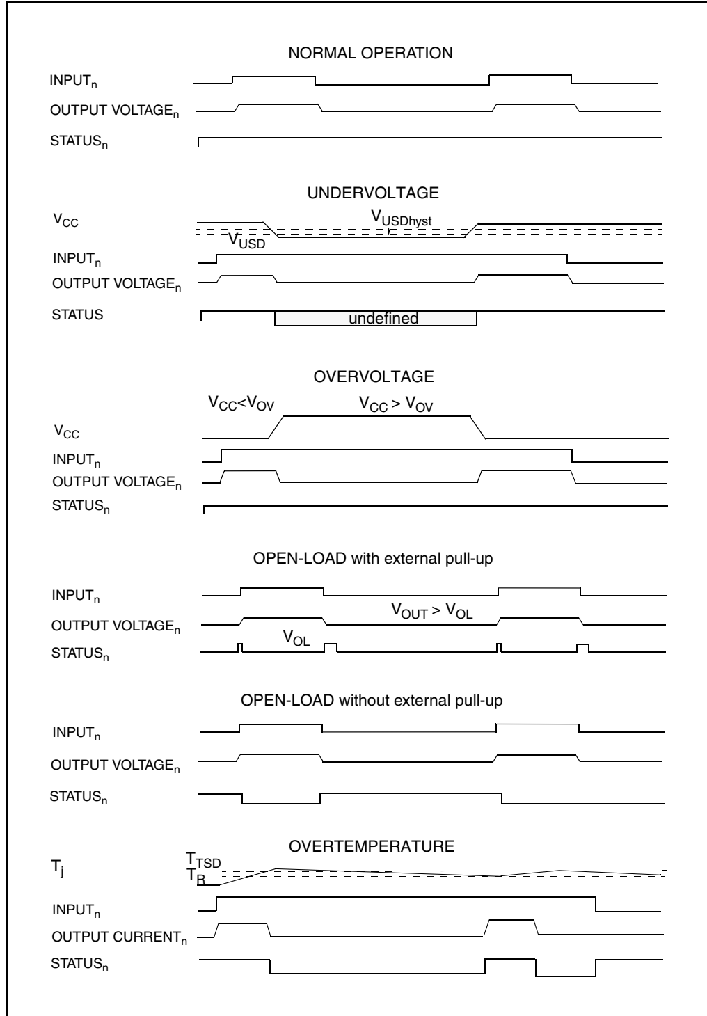
Figure 5. Waveforms
