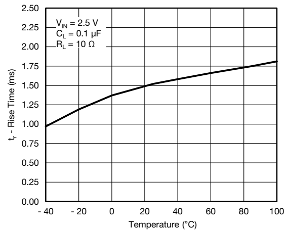
Rise Time vs. Temperature
