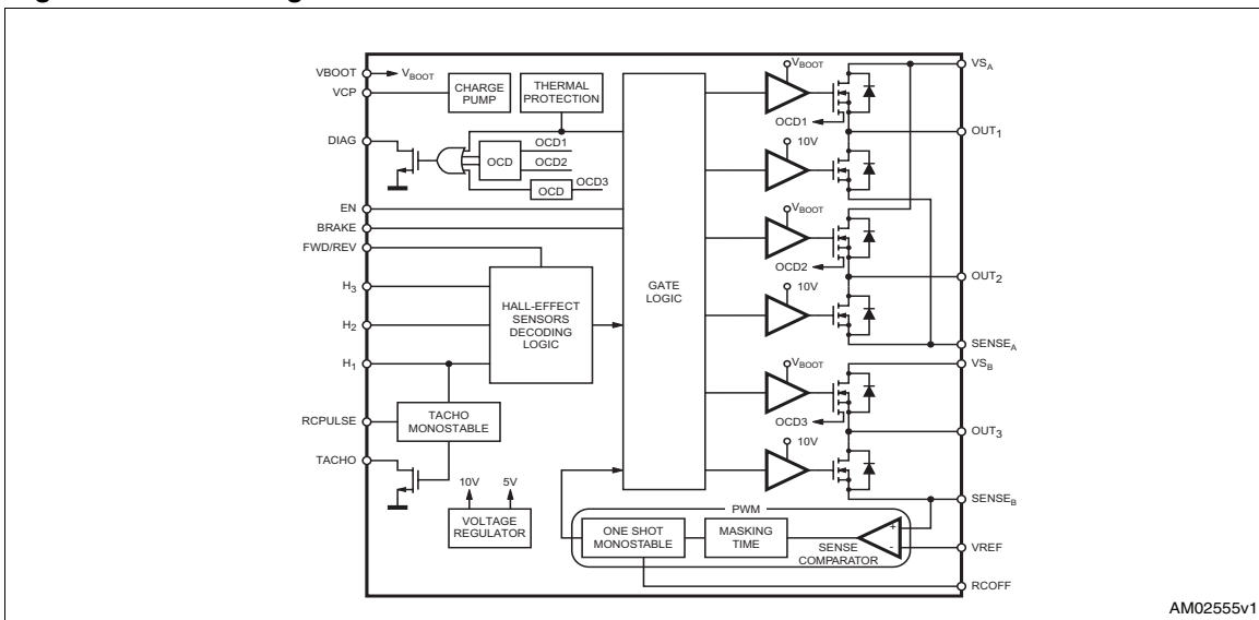
Figure 1. Block diagram
