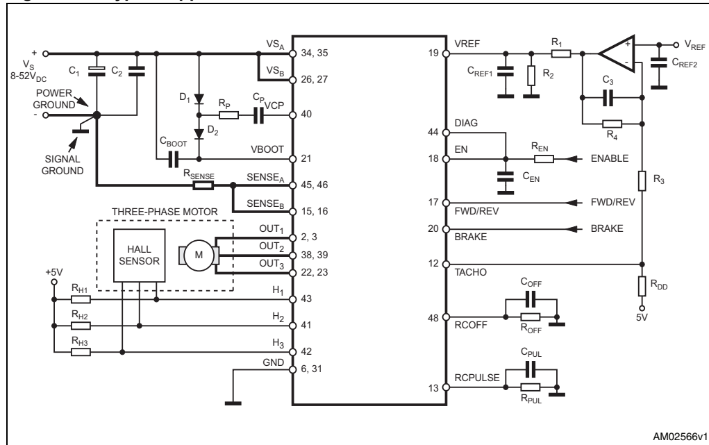
Figure 23. Typical application
