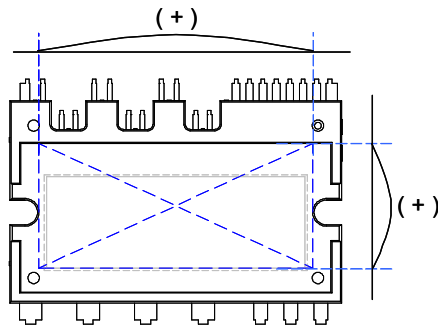
Figure 7. Flatness Measurement Position
