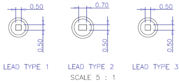
LEAD SECTION X-X'
