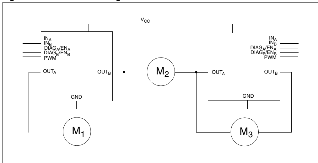
Figure 14. Multi-motors configuration
