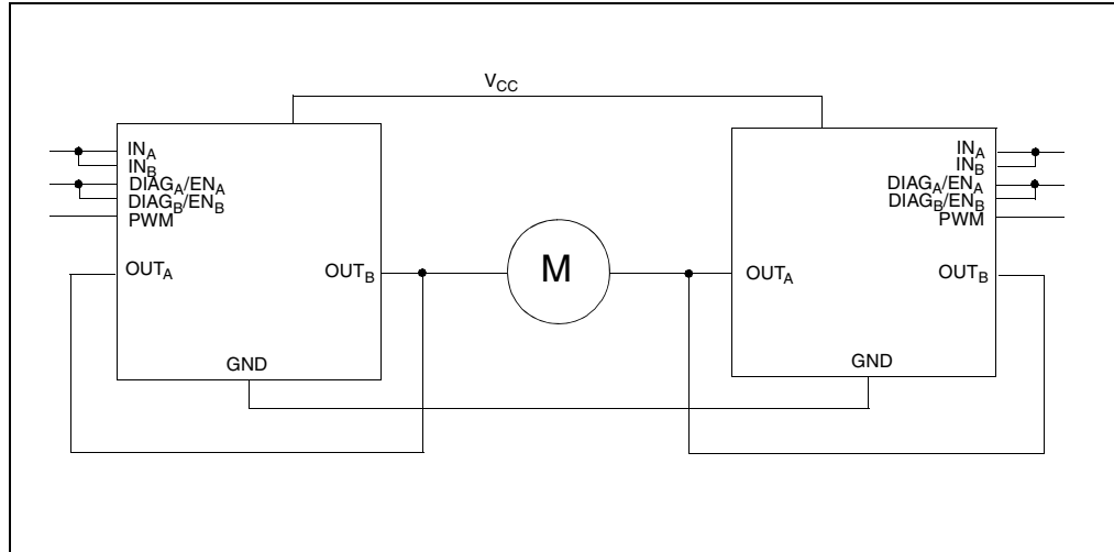
Figure 13. Half-bridge configuration
