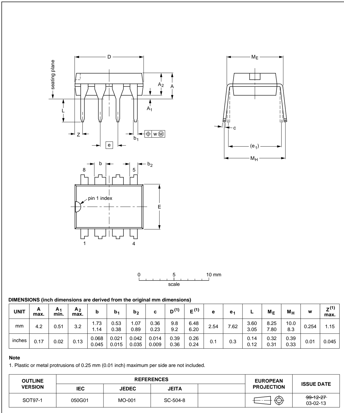
Fig 6. Package outline SOT97-1 (DIP8)
