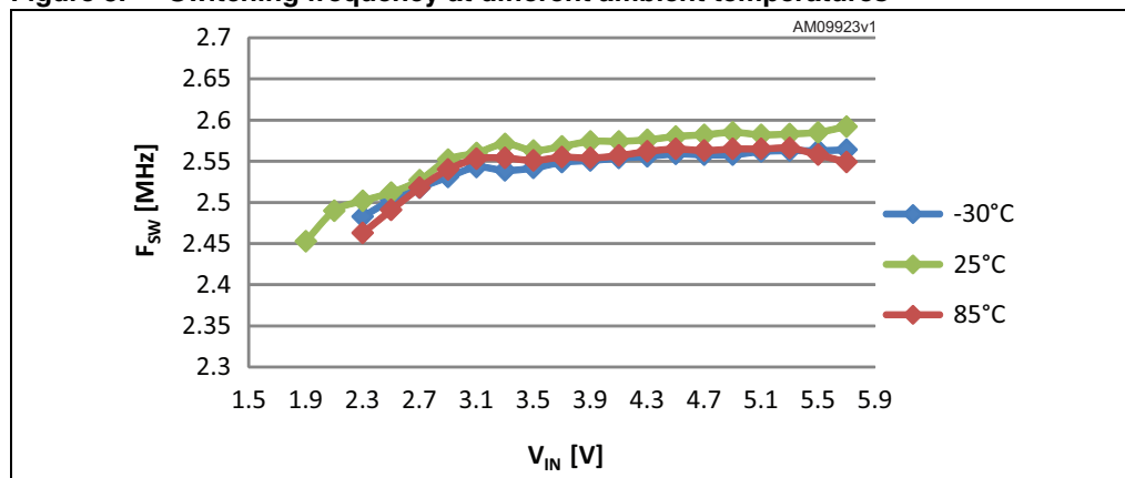
Figure 5. Switching frequency at different ambient temperatures
