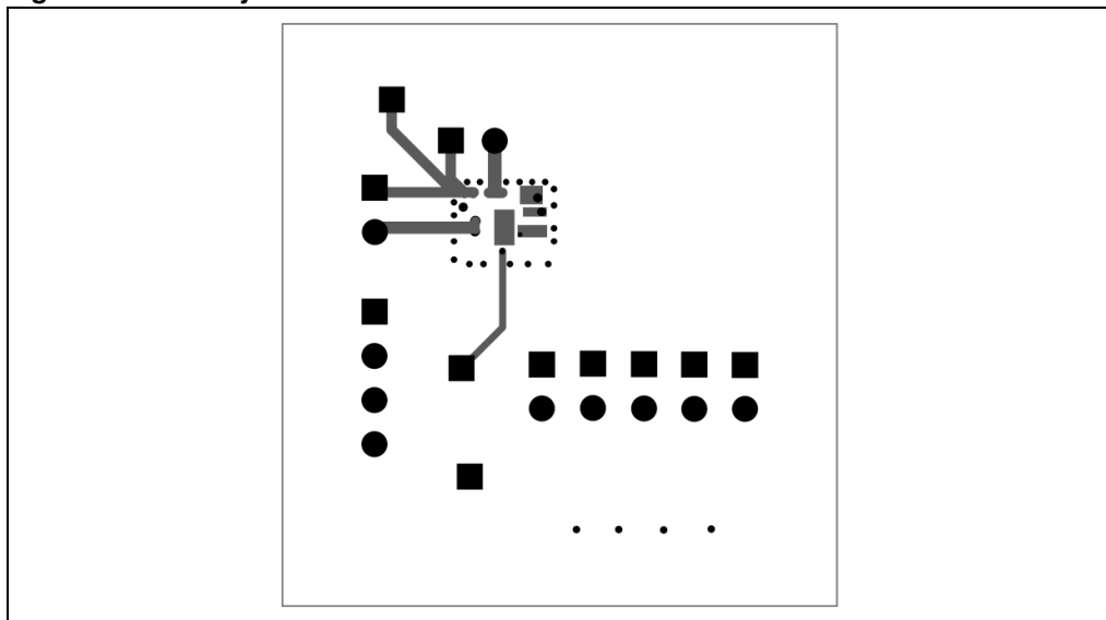
Figure 22. Mid layer 2
