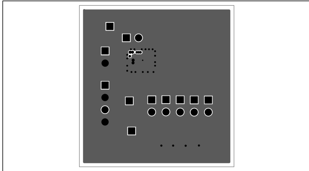
Figure 24. Top overlay
