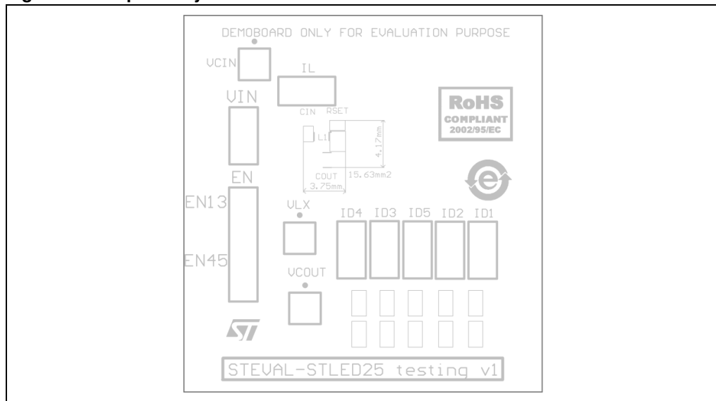
Figure 24. Top overlay
