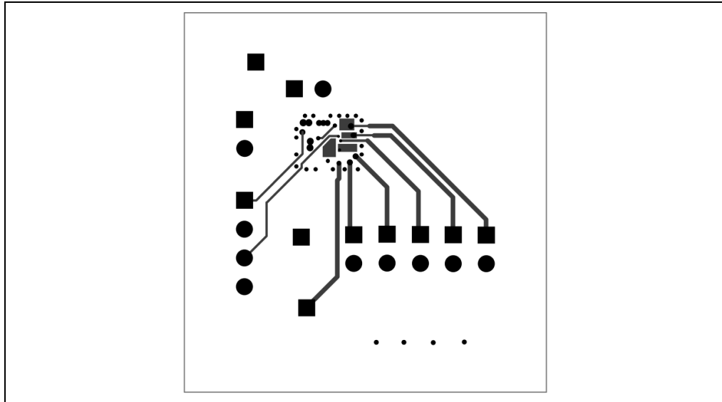
Figure 22. Mid layer 2
