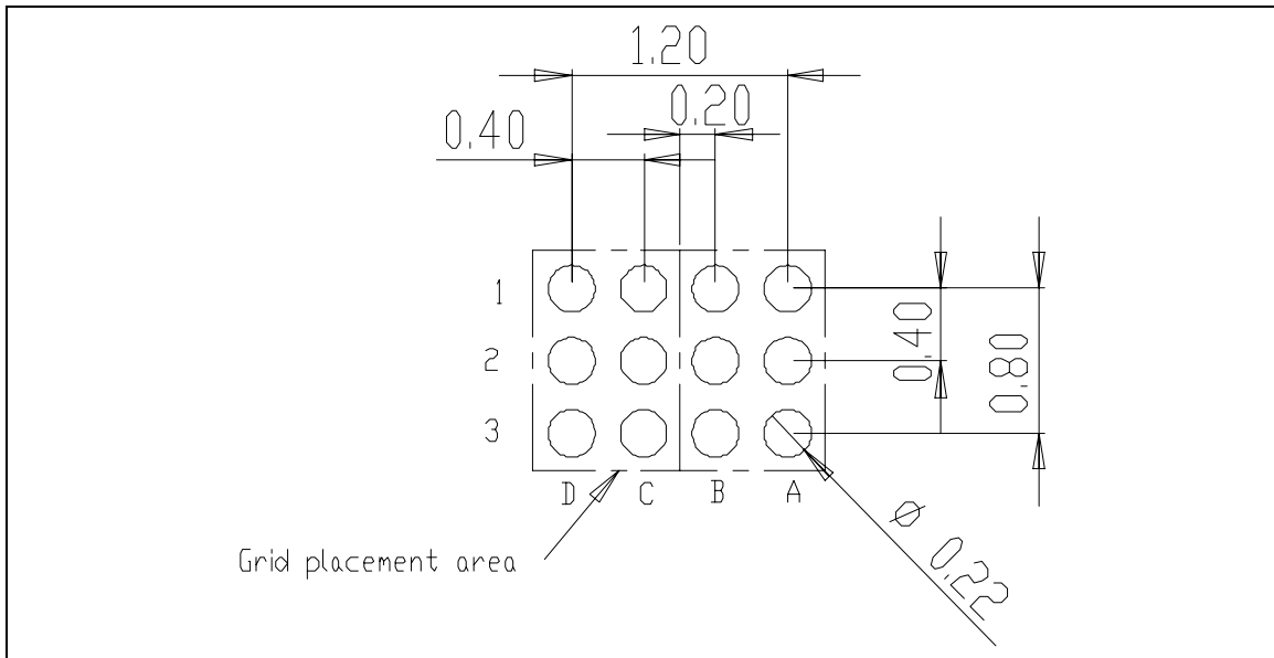
Figure 26. Footprint recommended data (mm.)
