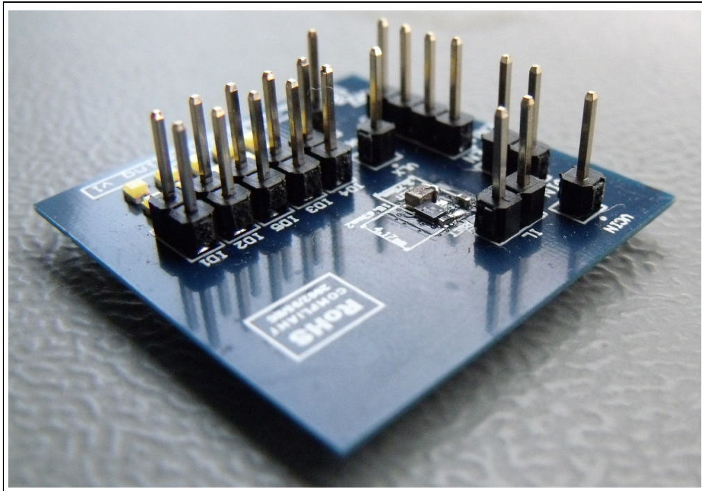
Figure 25. Photo of the application board
