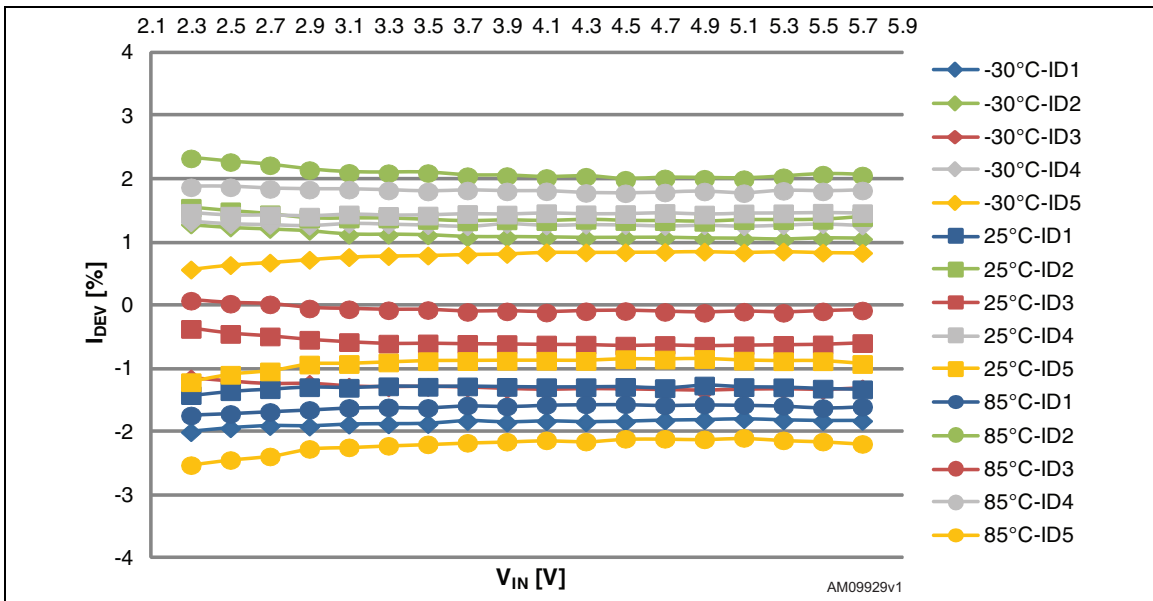
Figure 11. Current matching - set string current to 20 mA
