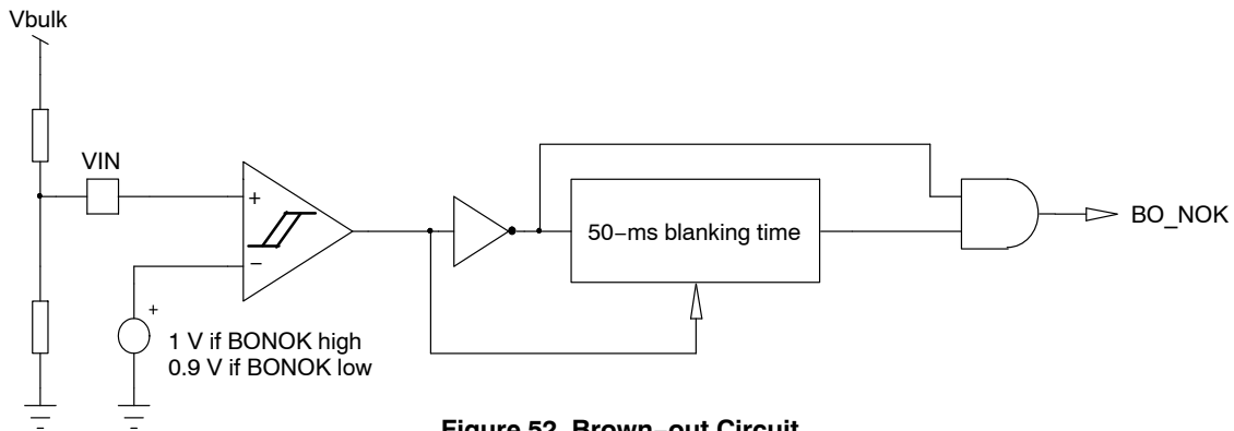
Figure 52. Brown-out Circuit
