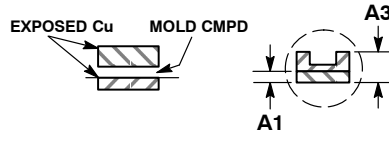
DETAIL B OPTIONAL CONSTRUCTIONS
