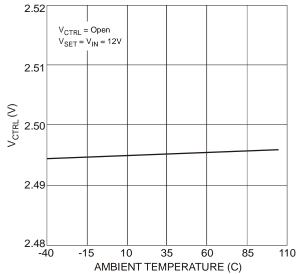
Figure 4 V_{CTRL} vs. Temperature
