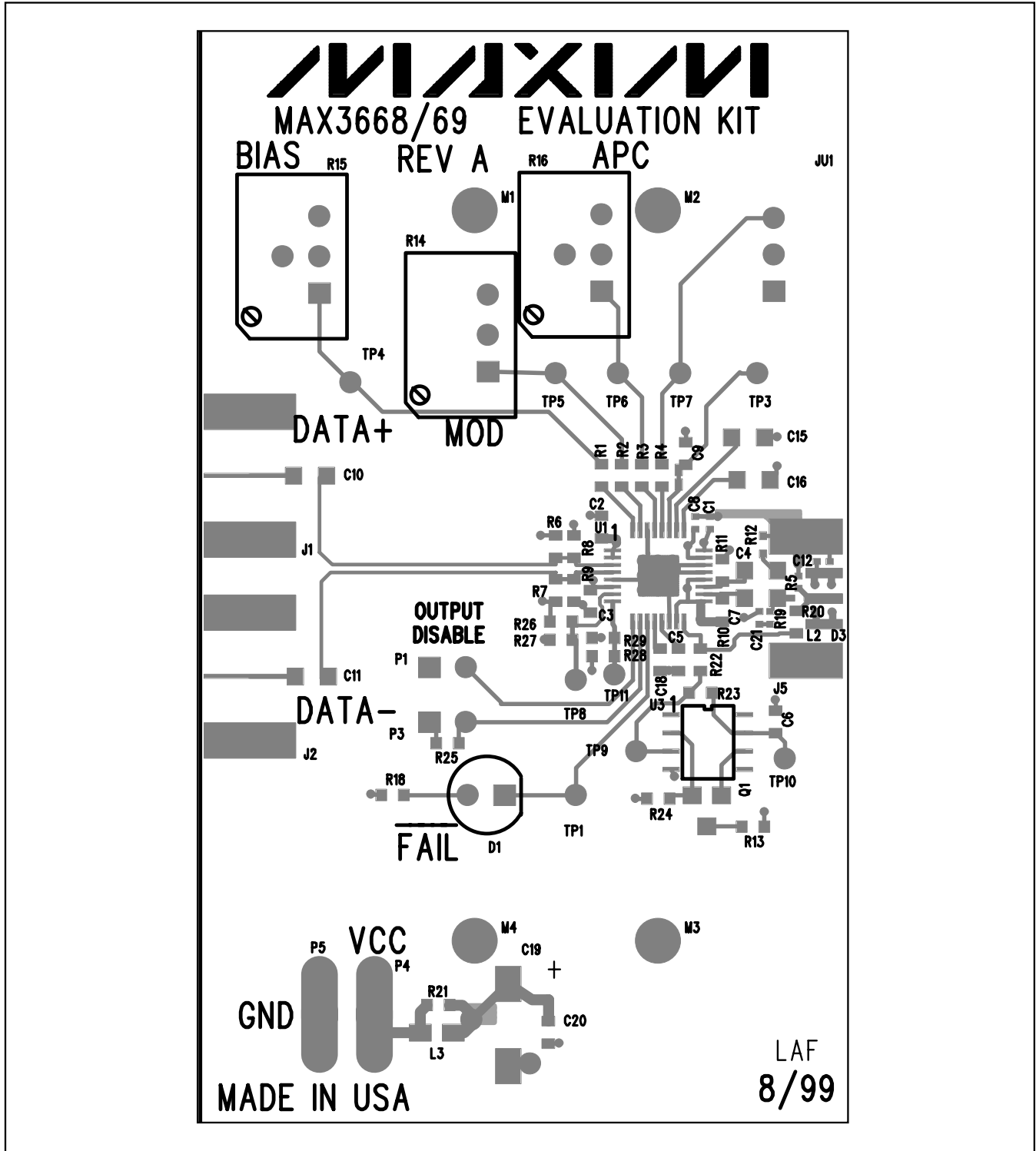
Figure 4a. MAX3669 EV Kit Component Placement Guide—Component Side
