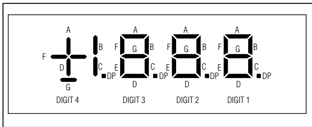
Figure 3. Segment Connection for the MAX1367 (3.5 Digits)
