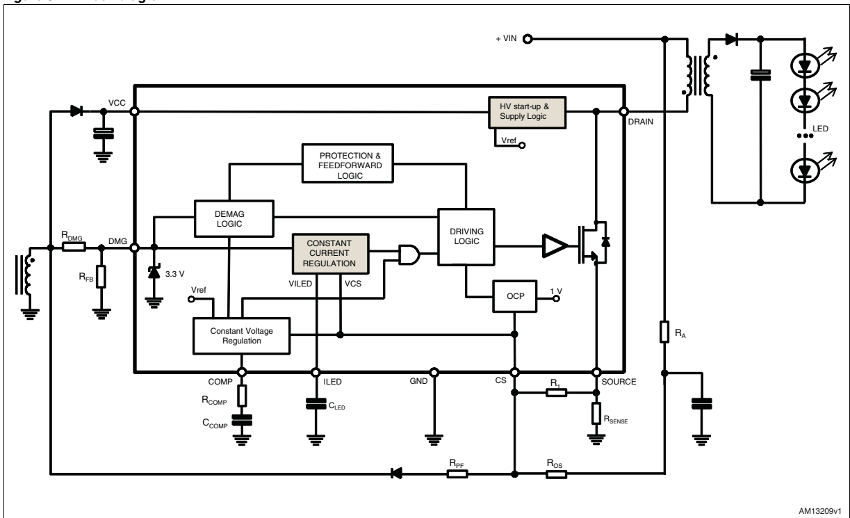
Figure 3. Block diagram
