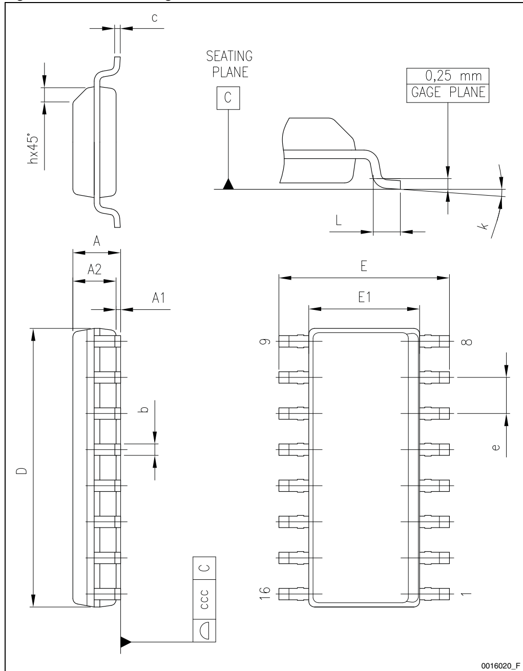
Figure 12. SO16N drawing
