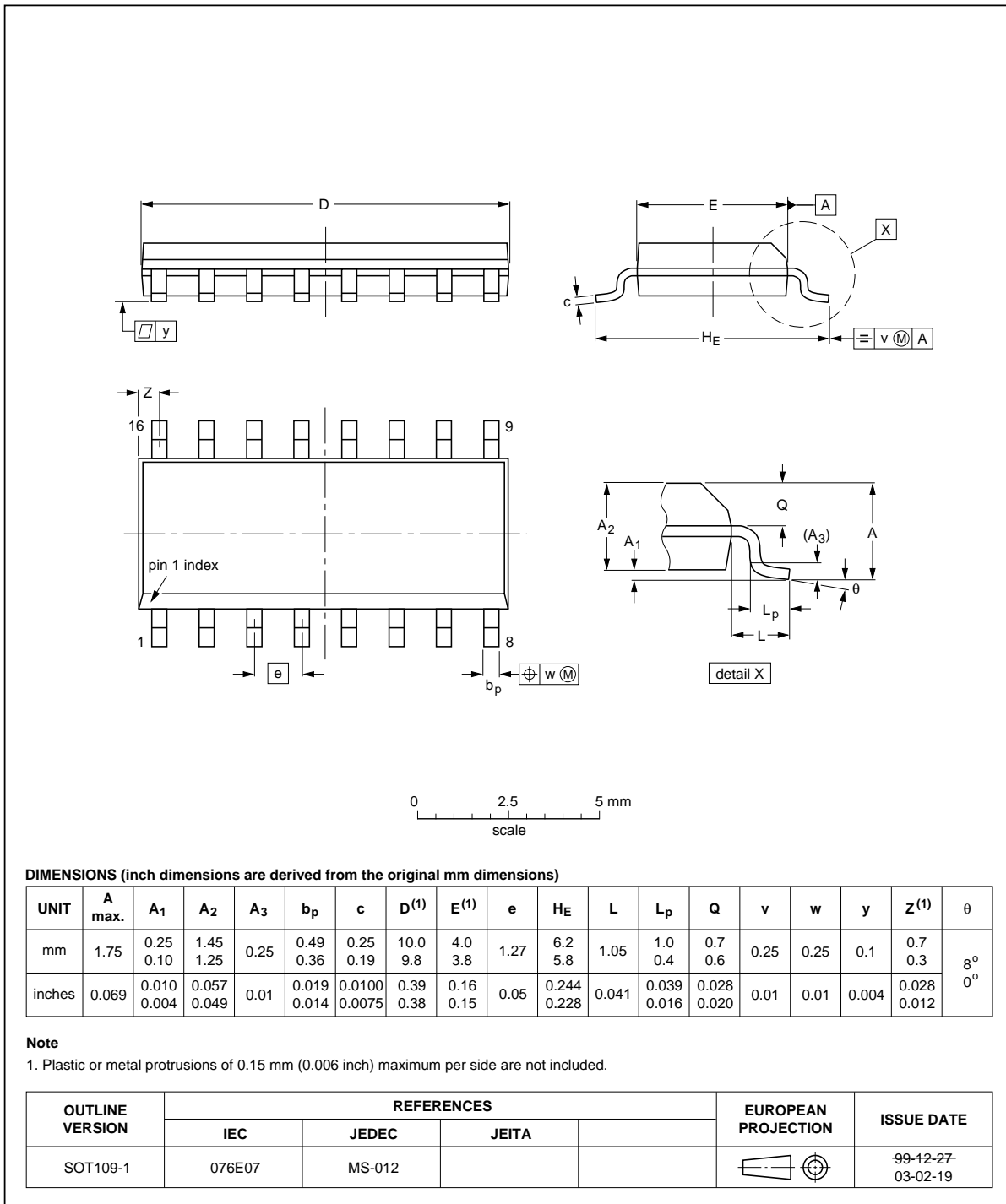
Fig 12. Package outline SOT109-1 (SO16)
