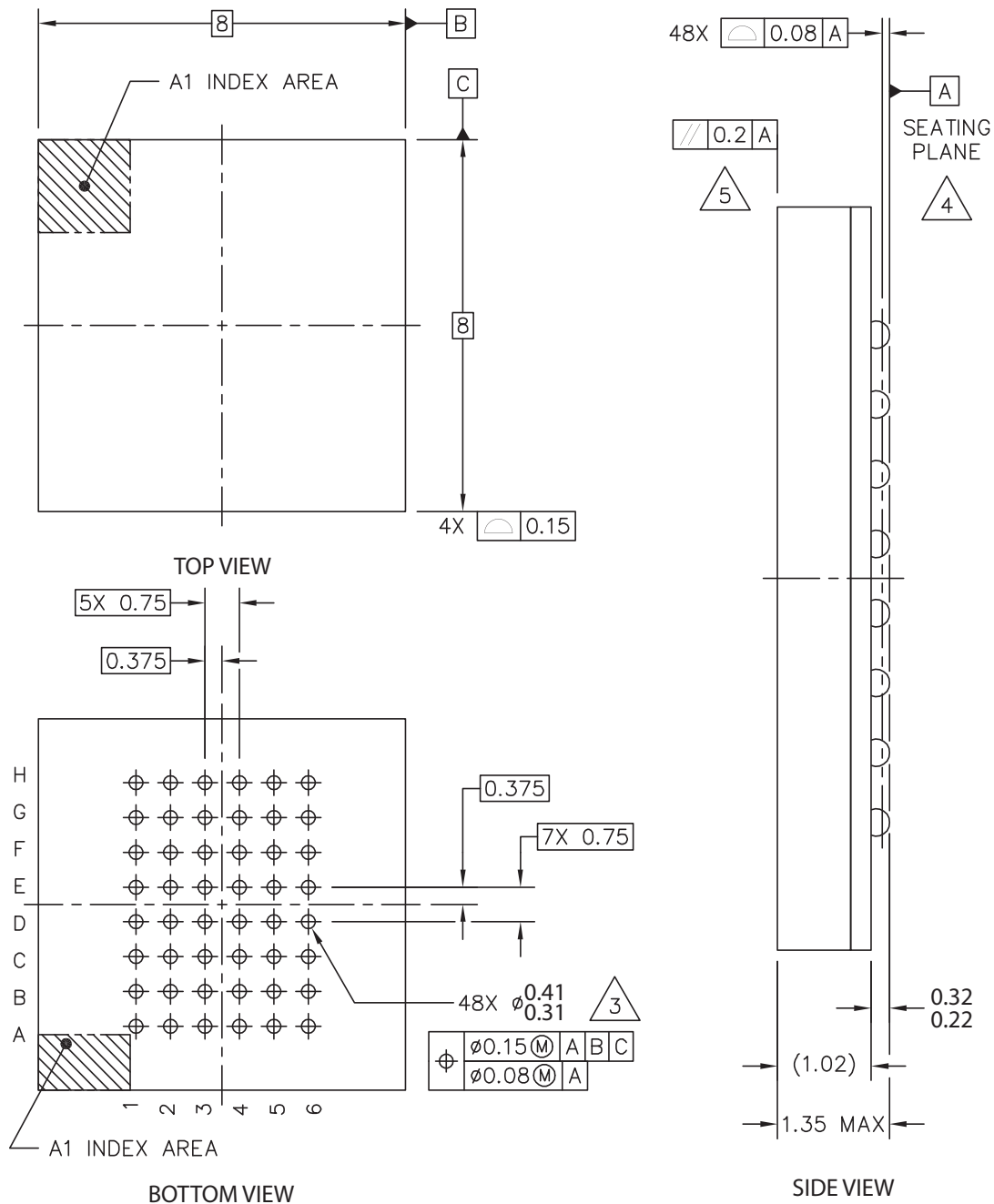
Figure 5.2 FBGA
