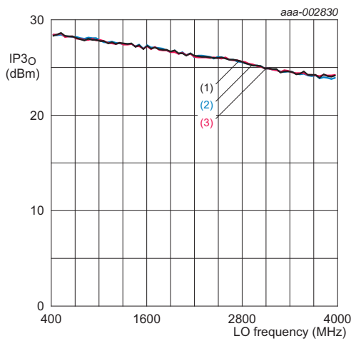
Fig 17. IP3_o versus f_{lo} and T_{mb}
