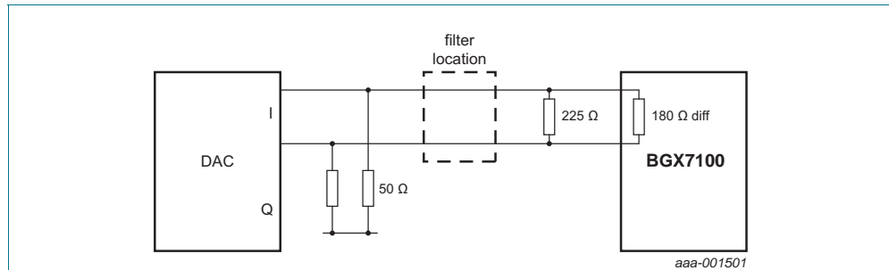
Fig 5. Typical low-power interface
