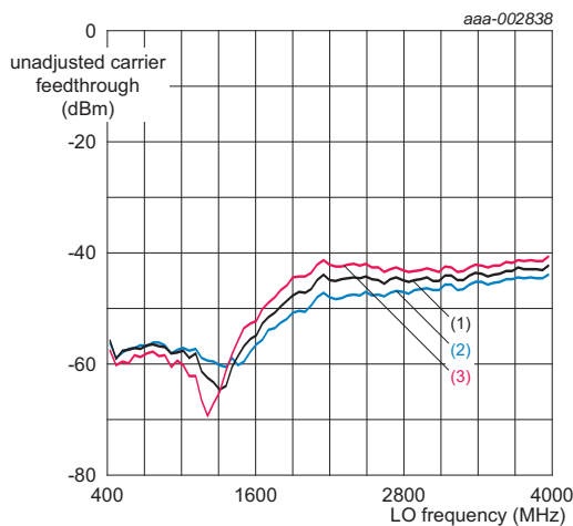
Fig 25. Unadjusted CF versus f_{lo} and T_{mb}
