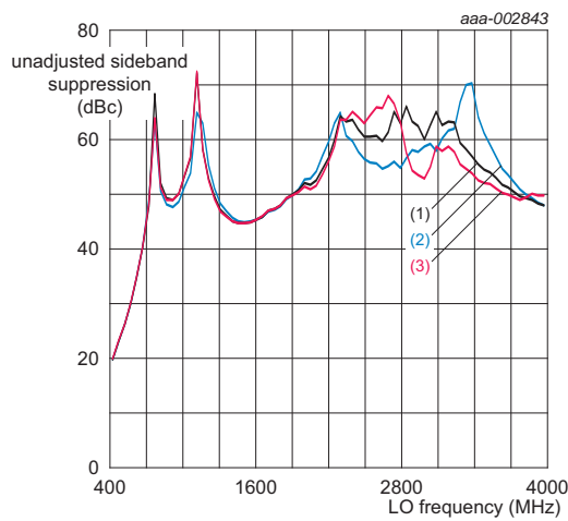
Fig 30. Unadjusted SBS versus f_{lo} and T_{mb}
