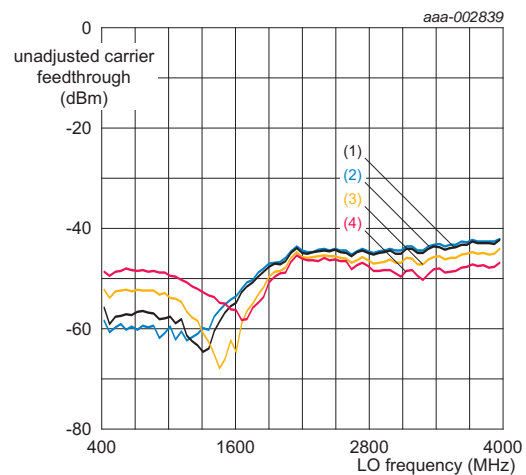
Fig 26. Unadjusted CF versus f_{lo} and V_{CC}
