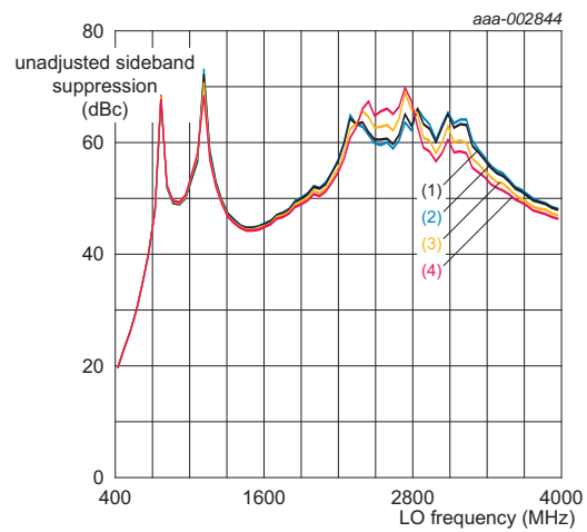
Fig 31. Unadjusted SBS versus f_{lo} and V_{CC}
