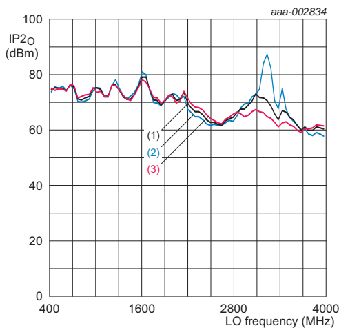
Fig 21. IP2_o versus f_{lo} and T_{mb}
