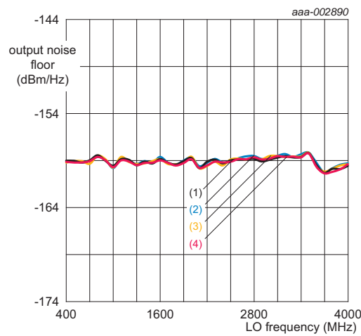
Fig 47. N_{flr(o)} versus f_{lo} and V_{CC}
