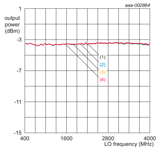
Fig 8. P_o versus f_{lo} and V_{CC}
