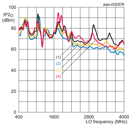
Fig 20. IP2_o versus f_{lo} and T_{mb}
