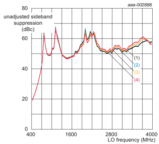
Fig 30. Unadjusted SBS versus f_{lo} and V_{CC}
