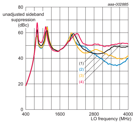
Fig 29. Unadjusted SBS versus f_{lo} and T_{mb}
