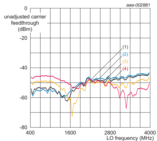
Fig 25. Unadjusted CF versus f_{lo} and V_{CC}
