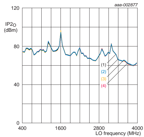
Fig 21. IP2_o versus f_{lo} and V_{CC}
