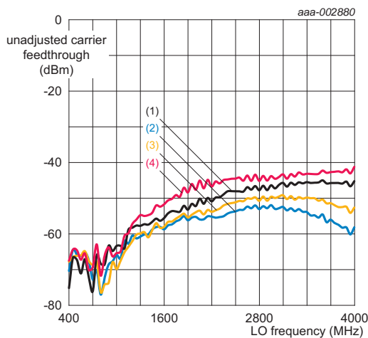
Fig 24. Unadjusted CF versus f_{lo} and T_{mb}
