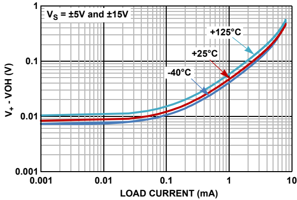
FIGURE 23. OUTPUT OVERHEAD VOLTAGE HIGH vs LOAD CURRENT, -40^\circ C to +125^\circ C , V_S = \pm 5V AND \pm 15V
