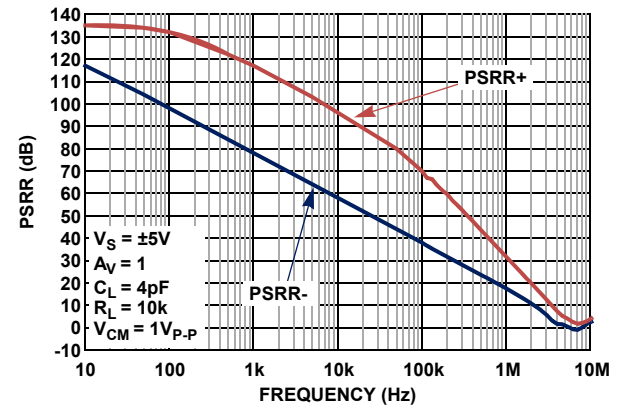
FIGURE 14. PSRR vs FREQUENCY, V_S = \pm 5V
