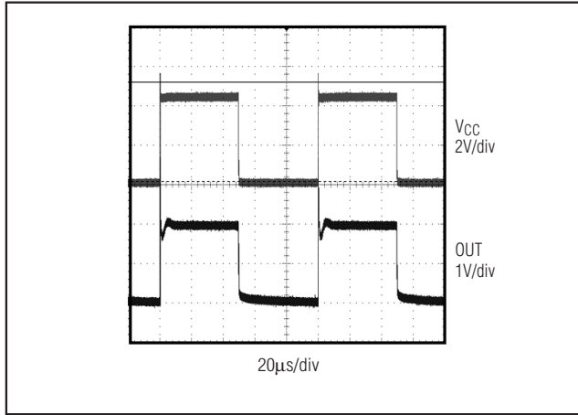
Figure 6. Power-Up/Power-Down Waveform
