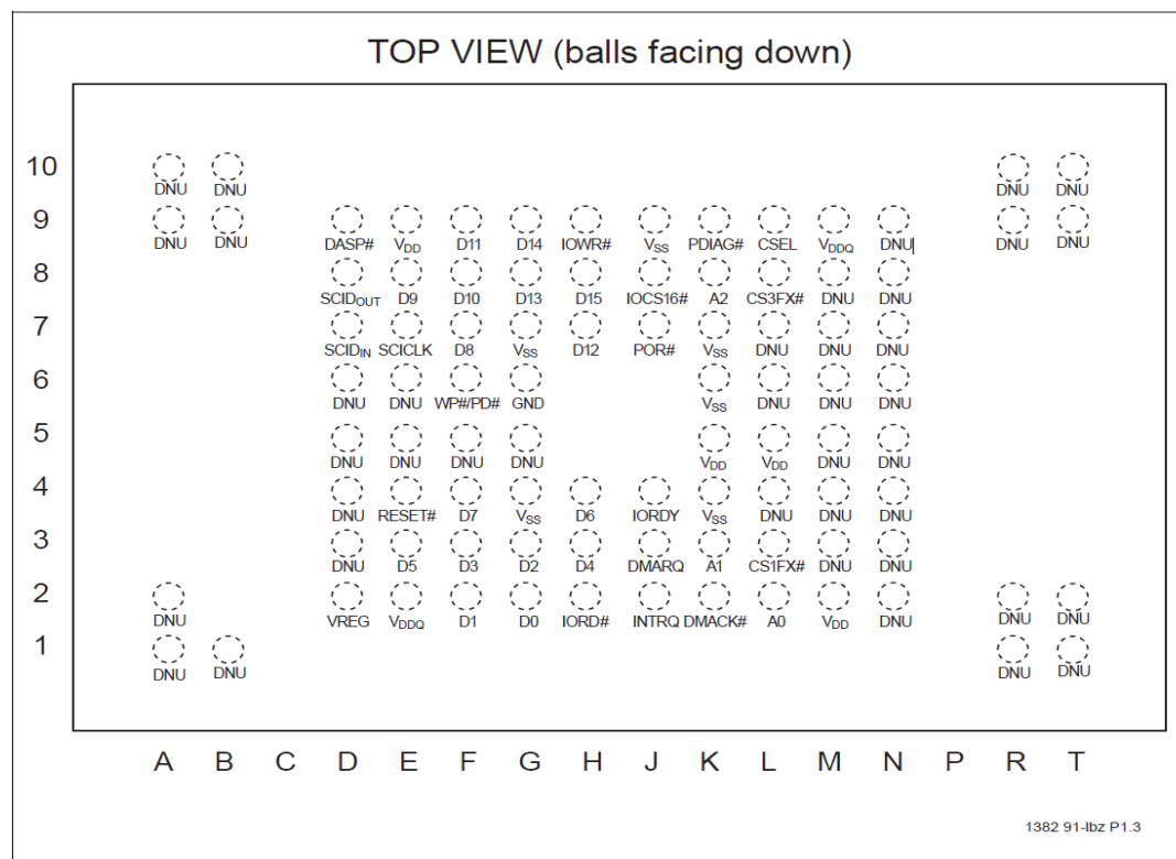
Figure 3-1: Pin Assignments for 91-Ball LBGA
