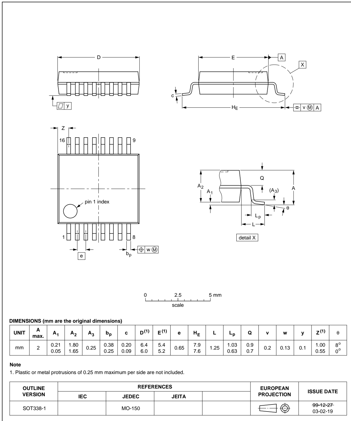
Fig 10. Package outline SOT338-1 (SSOP16)
