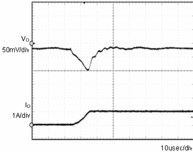
Fig.3 Transient Response (0→1.0A) C_o=1\mu\text{F}
