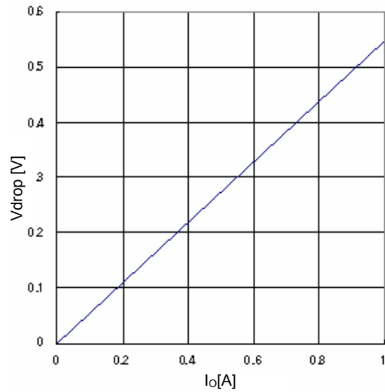
Fig.22 Minimum dropout Voltage 2 ( V_{CC}=4.5V , T_a=25^{\circ}C )
