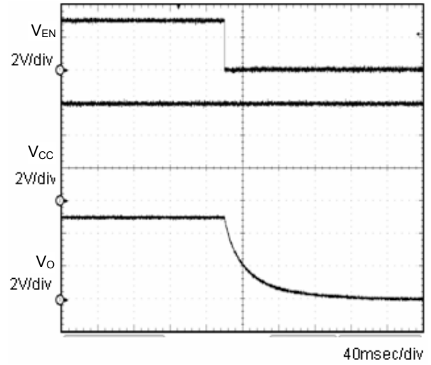
Fig.8 OFF sequence 2 C_o=1\mu F
