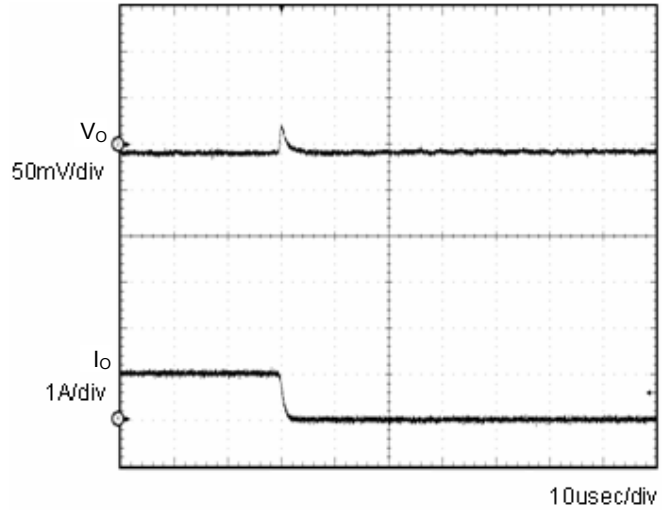
Fig.4 Transient Response (1.0→0A) C_o=1\mu\text{F}
