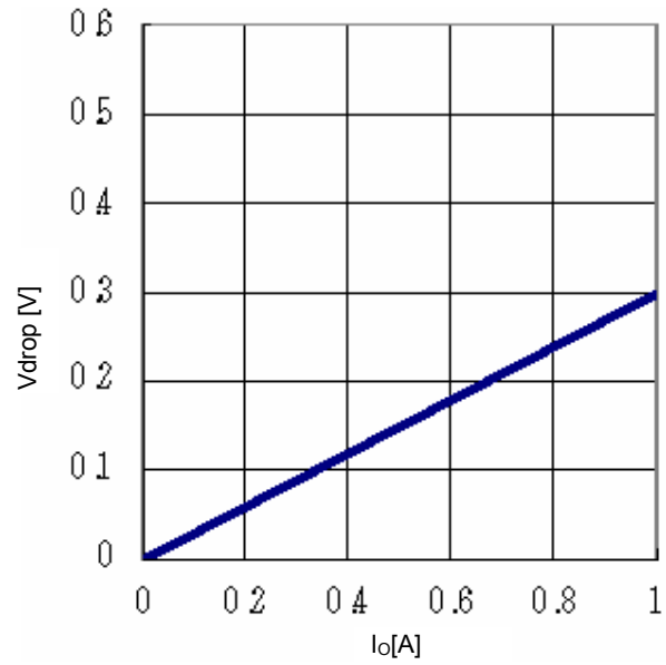
Fig.26 Minimum dropout Voltage 6 ( V_{CC}=12V , T_a=25^\circ C )
