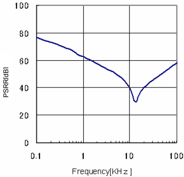
Fig.21 PSRR ( I_o=0mA )
