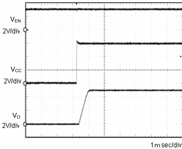
Fig.5 Input sequence 1 C_o=1\mu\text{F}
