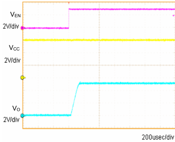
Fig.7 Input sequence 2 C_o=1\mu F
