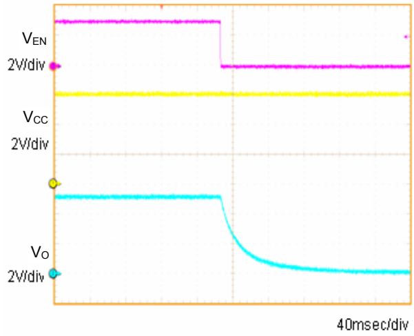
Fig.8 OFF sequence 2 C_o=1\mu F
