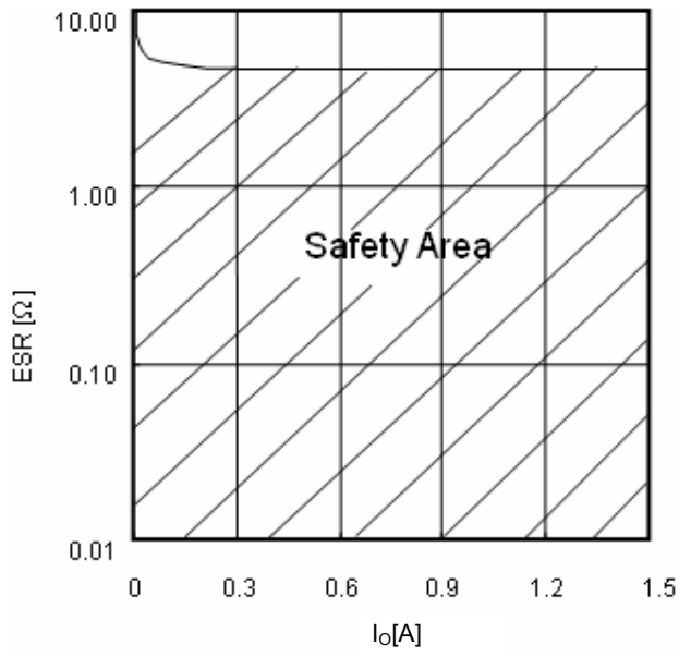
Fig.19 ESR condencer
