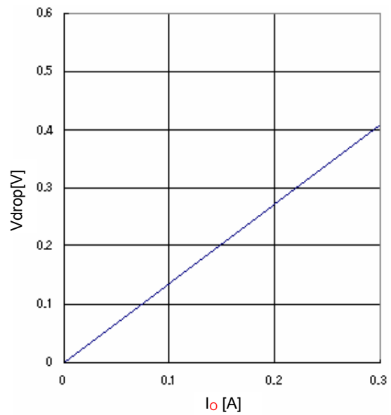
Fig.22 Minimum dropout Voltage 2 ( V_{CC}=4.5V , T_a=25^{\circ}C )
