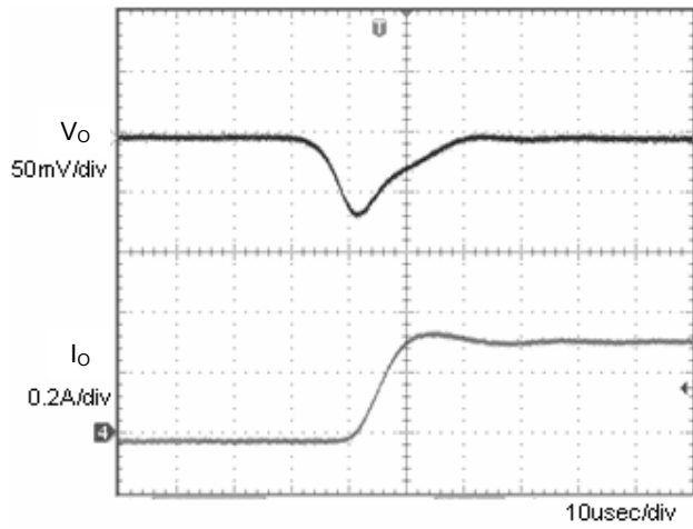
Fig.3 Transient Response (0→0.3A) Co=1µF
