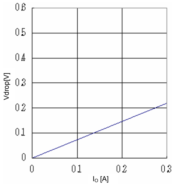
Fig.26 Minimum dropout Voltage 6 ( V_{CC}=12V , T_a=25^\circ C )
