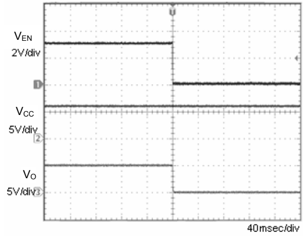
Fig.8 OFF sequence 2 Co=1μF
