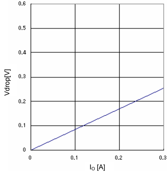
Fig.24 Minimum dropout Voltage 4 ( V_{CC}=8V , T_a=25^\circ C )
