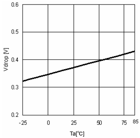
Fig.18 Minimum dropout Voltage1 ( V_{CC}=5V, I_o=0.3A )
