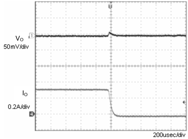
Fig.4 Transient Response (0.3→0A) Co=1µF
