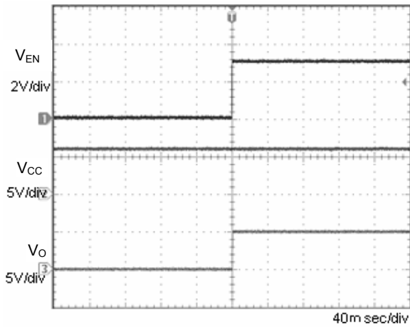
Fig.5 Input sequence 1 Co=1µF
