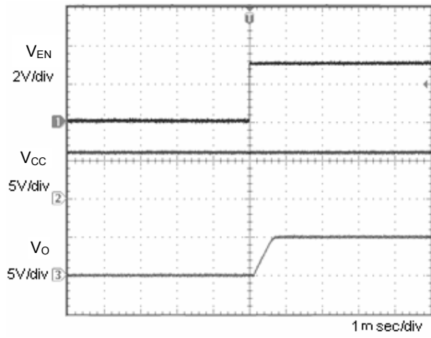
Fig.7 Input sequence 2 Co=1μF
