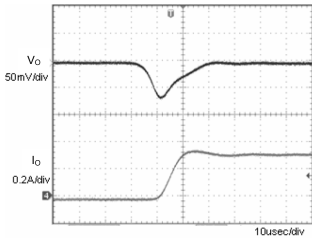
Fig.3 Transient Response (0→0.3A) C_o=1\mu\text{F}
