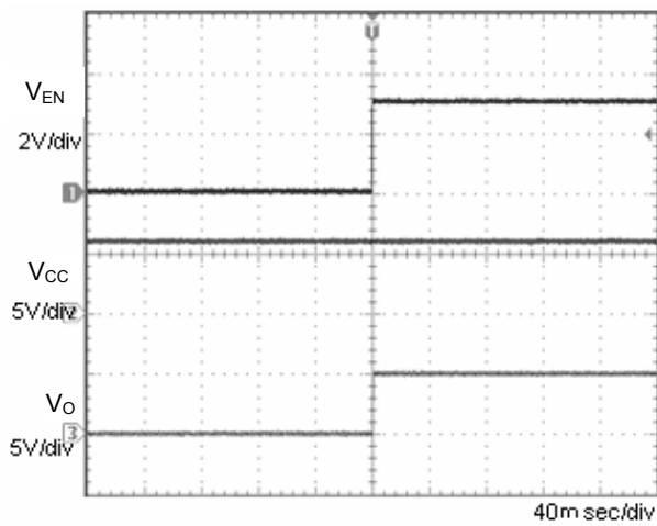
Fig.5 Input sequence 1 C_o=1\mu\text{F}
