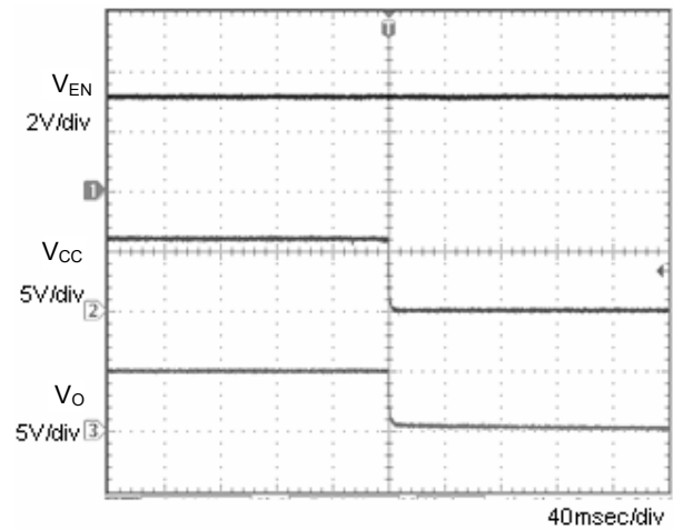
Fig.6 OFF sequence 1 C_o=1\mu\text{F}
