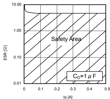
ESR – I_O characteristics
