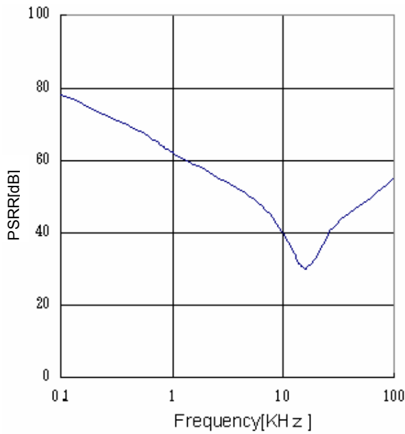
Fig.21 PSRR ( I_o=0mA )
