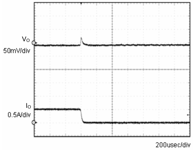
Fig.4 Transient Response (0.5→0A) Co=1µF
