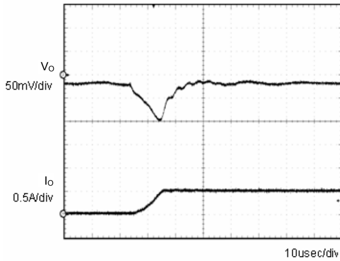
Fig.3 Transient Response (0→0.5A) Co=1µF
