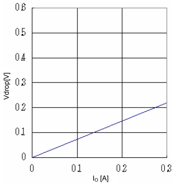
Fig.26 Minimum dropout Voltage 6 ( V_{CC}=12V , T_a=25^\circ C )
