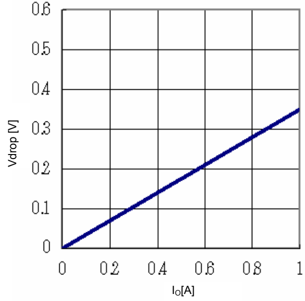
Fig.24 Minimum dropout Voltage 4 (V CC =8V, Ta=25°C)
