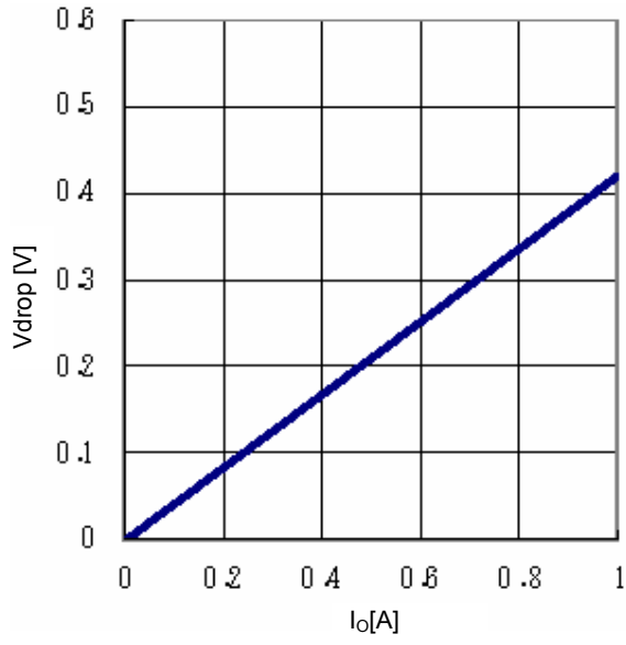
Fig.23 Minimum dropout Voltage 3 (V CC =6V, Ta=25°C)
