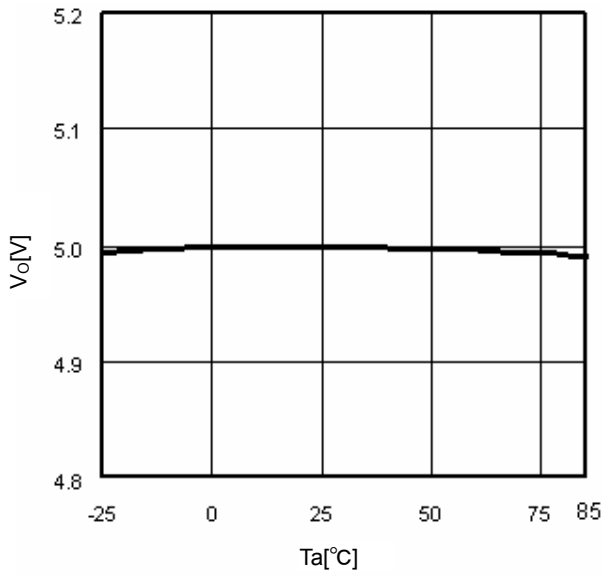
Fig.9 T_a - V_O ( I_o = 0\text{mA} )
