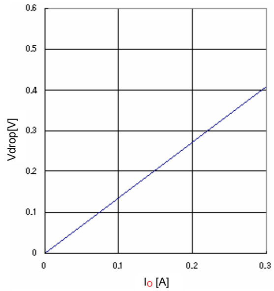
Fig.22 Minimum dropout Voltage 2 ( V_{CC}=4.5\text{V} , T_a=25^\circ\text{C} )
