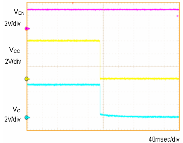
Fig.6 OFF sequence 1 Co=1μF
