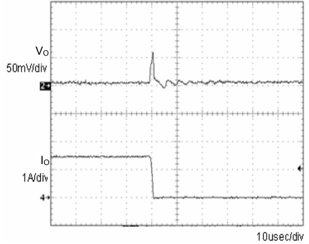
Fig.4 Transient Response (1.5→0A) Co=1μF
