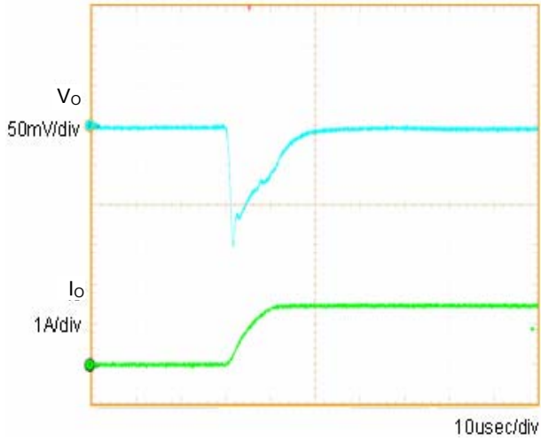
Fig.3 Transient Response (0→1.5A) Co=1μF
