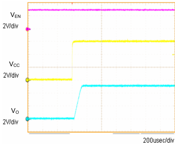
Fig.5 Input sequence 1 Co=1μF
