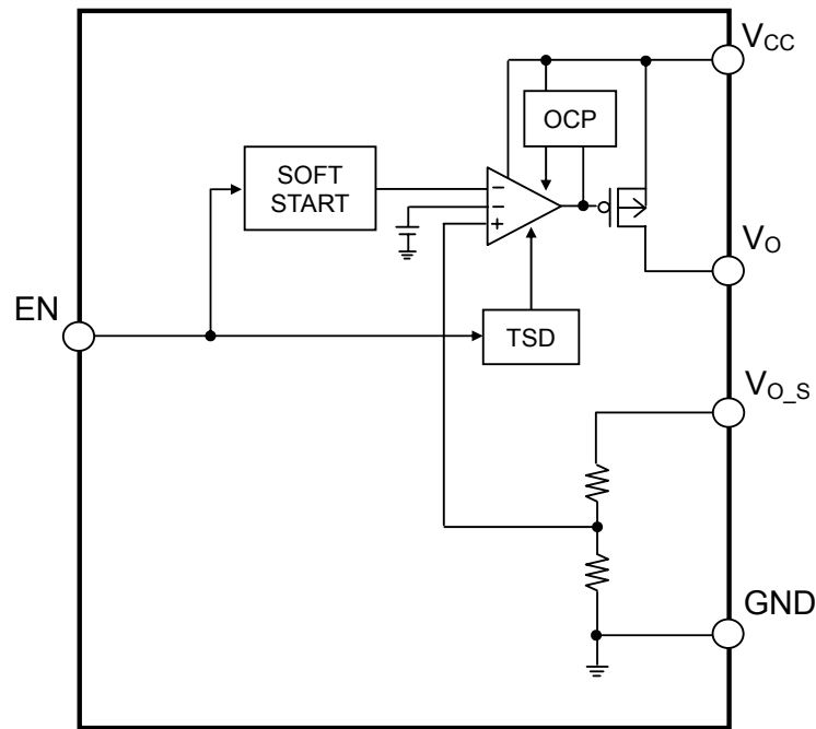
Fig.2 Block Diagram
