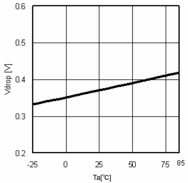
Fig.18 Minimum dropout Voltage1 ( V_{cc}=5V, I_o=-0.5A )
