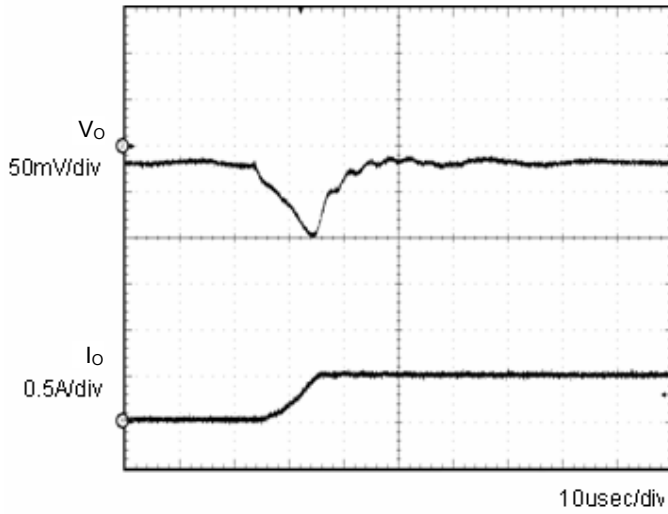
Fig.3 Transient Response (0→0.5A) C_o=1\mu\text{F}
