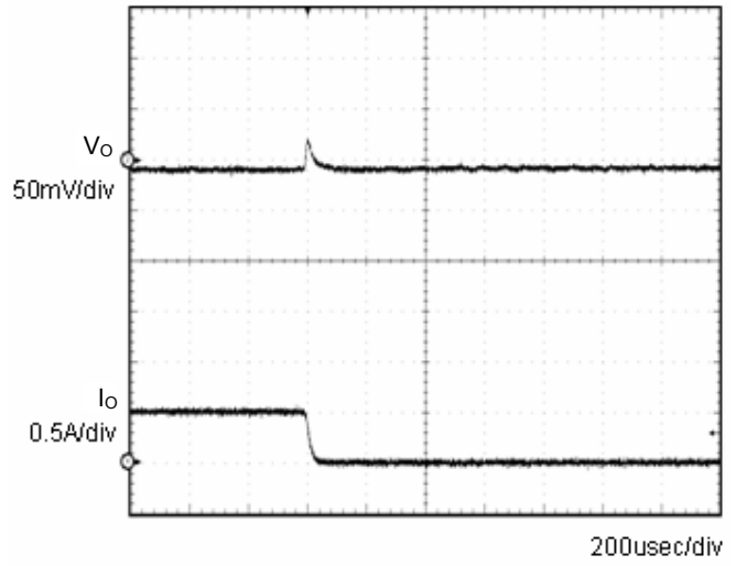
Fig.4 Transient Response (0.5→0A) C_o=1\mu\text{F}
