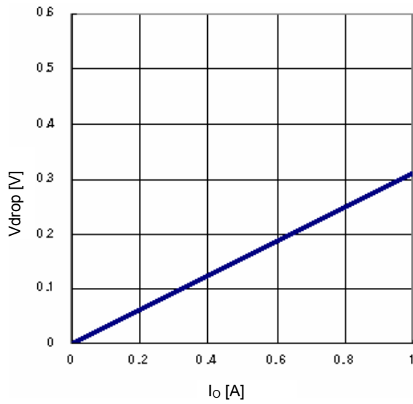
Fig.25 Minimum dropout Voltage 5 ( V_{CC}=10V , T_a=25^{\circ}C )
