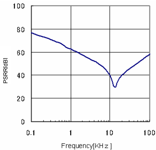
Fig.21 PSRR ( I_o=0mA )
