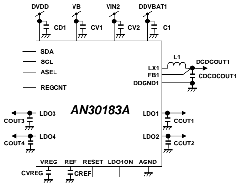
Figure : Application Circuit
