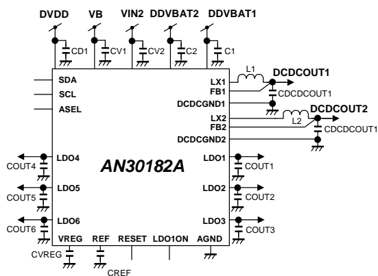
Figure : Application Circuit
