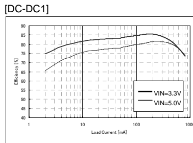
Condition : VIN=3.3V, 5.0V, Vout=1.2V, Cout=10µF, Lout=2.2µH
