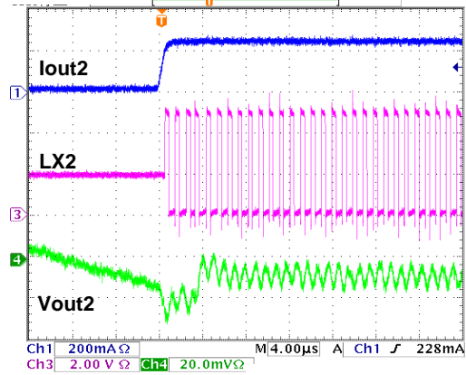
DC-DC2 Iout2 = 10 mA to 250 mA , Δ t = 1 μsec
