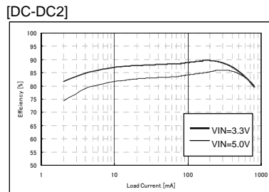
Condition : VIN=3.3V, 5.0V, Vout=1.8V, Cout=10µF, Lout=2.2µH
