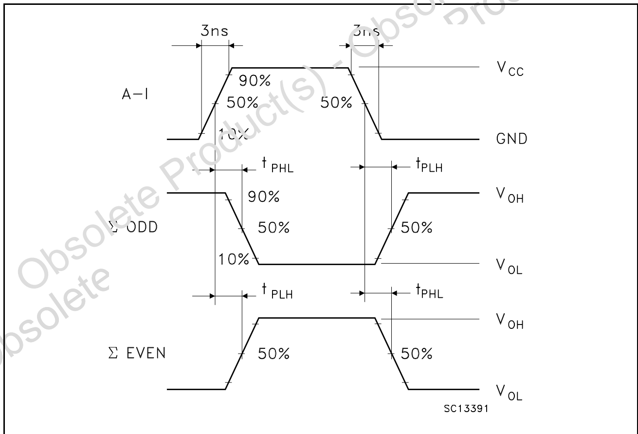
Figure 5: Waveform - Propagation Delays ( f=1\text{MHz} ; 50% duty cycle)
