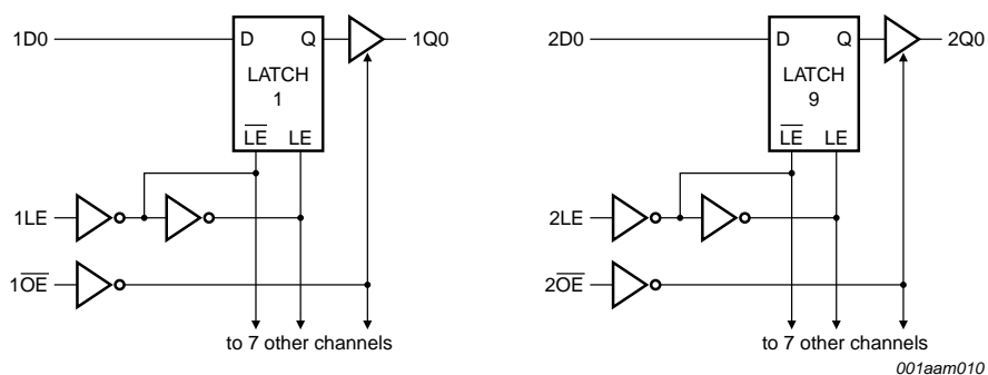
Fig 4. Logic diagram
